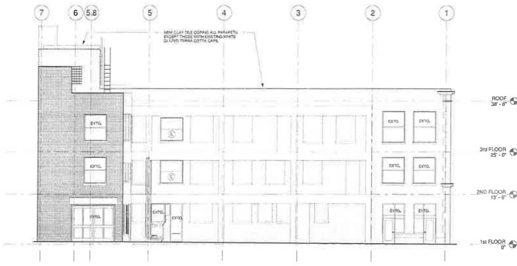
② EAST ELEVATION 1/8" = 1'-0"
