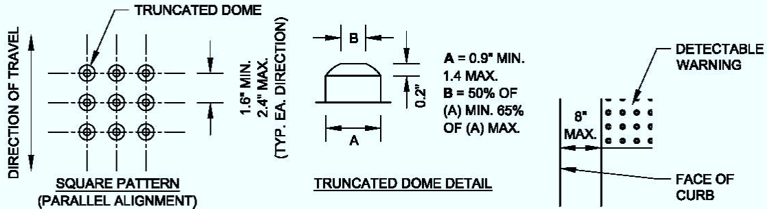
UNIT PATTERN & DOME DETAIL
