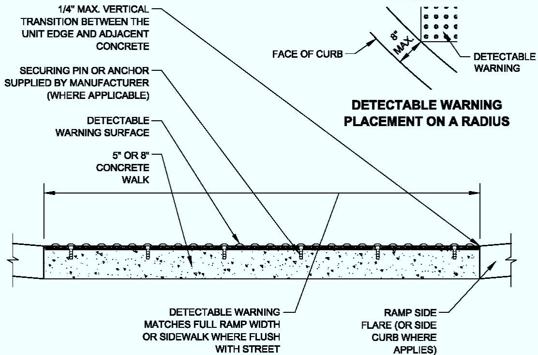
TYPICAL DETECTABLE WARNING PLACEMENT
