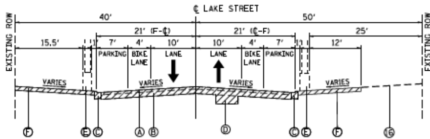
EXISTING TYPICAL CROSS SECTION STA 60+55.00 TO STA 63+47.82
