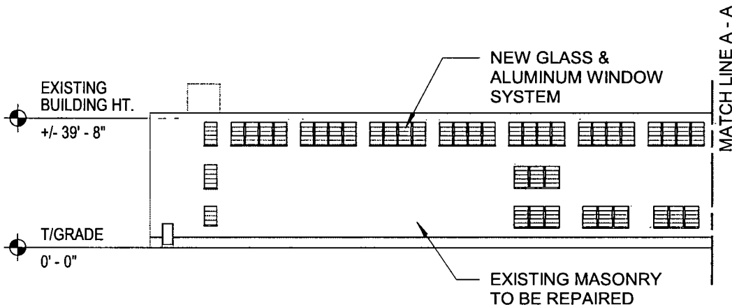
EAST ELEVATION - SOUTH PORTION
