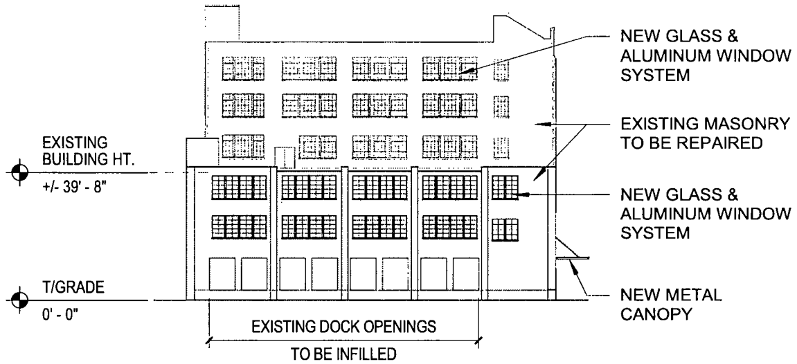
SOUTH ELEVATION
