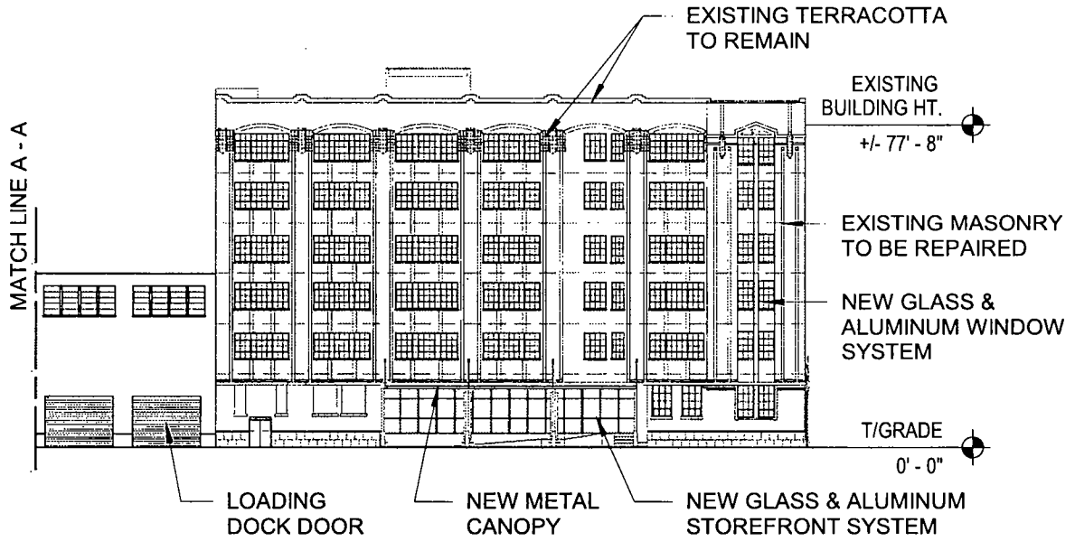
EAST ELEVATION - NORTH PORTION
