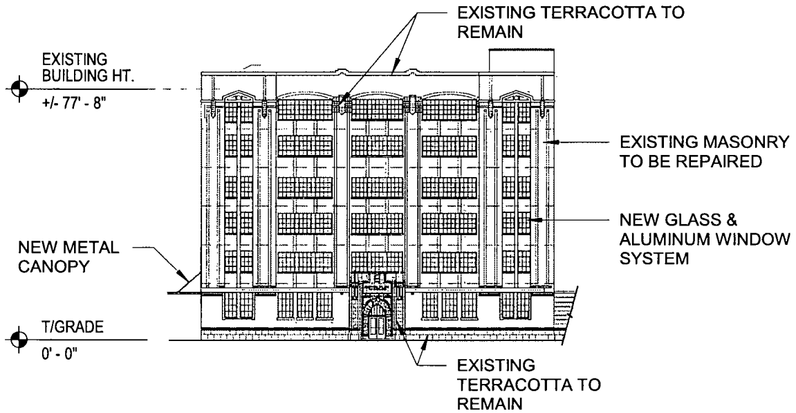
NORTH ELEVATION
