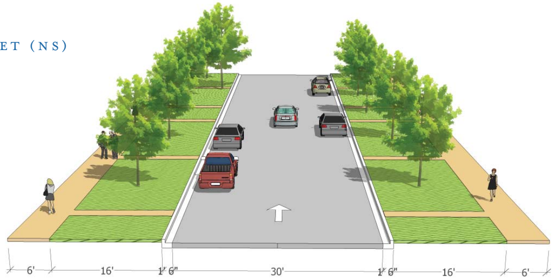
EXISTING CROSS-SECTION AND DIMENSIONING OF ST LAWRENCE AVENUE
