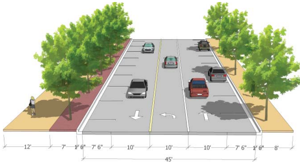
PROPOSED CROSS-SECTION AND DIMENSIONING OF MARTIN LUTHER KING DRIVE
