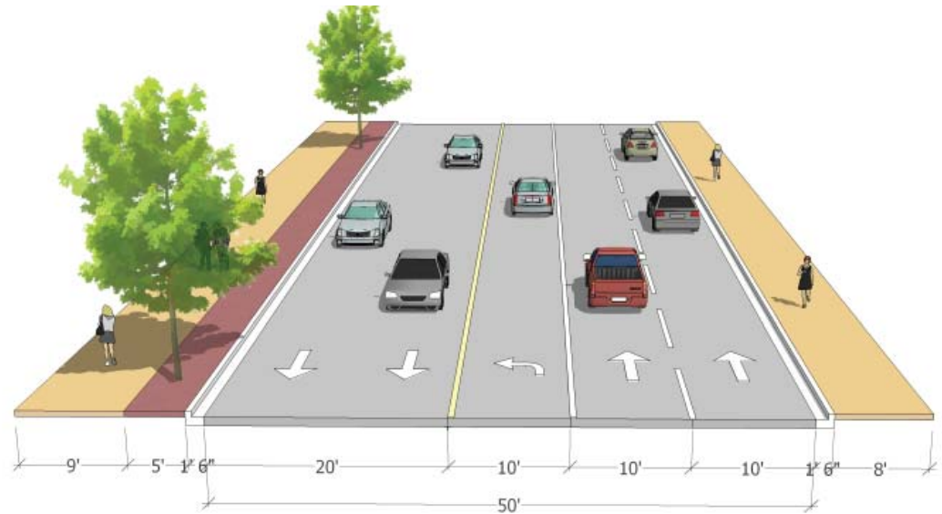
EXISTING CROSS-SECTION AND DIMENSIONING OF MARTIN LUTHER KING DRIVE
