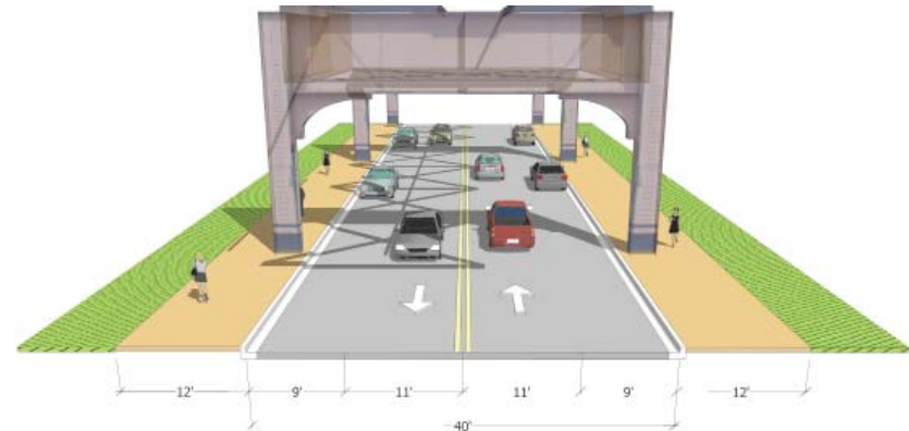
EXISTING CROSS-SECTION AND DIMENSIONING OF 63RD STREET
