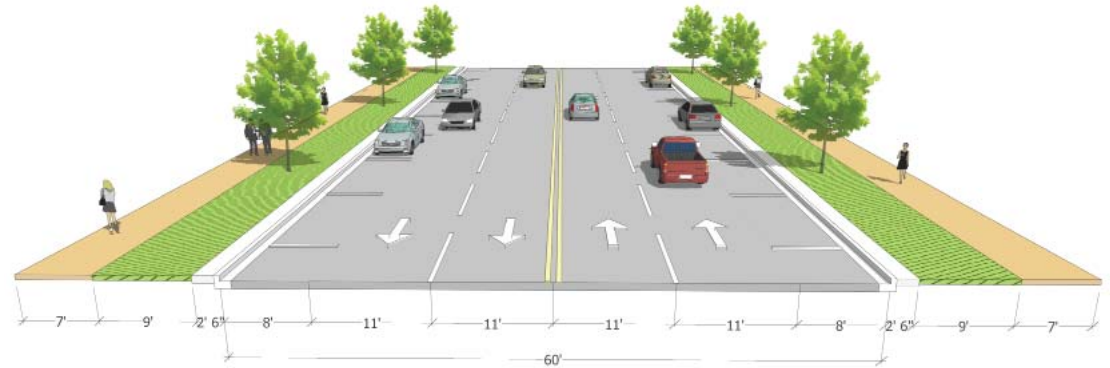
EXISTING CROSS-SECTION AND DIMENSIONING OF COTTAGE GROVE AVENUE.
