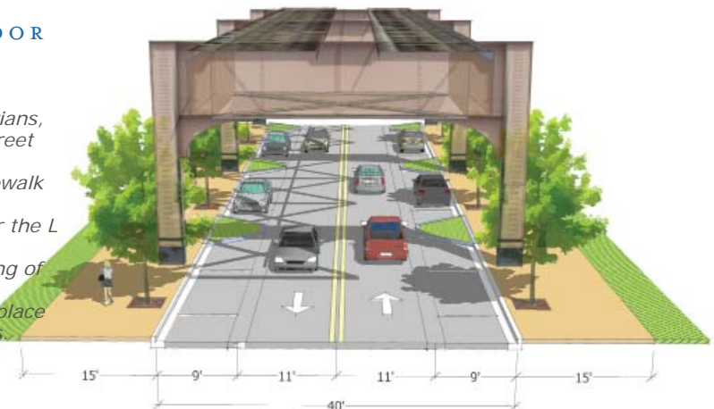
PROPOSED CROSS-SECTION AND DIMENSIONING OF 63RD STREET
