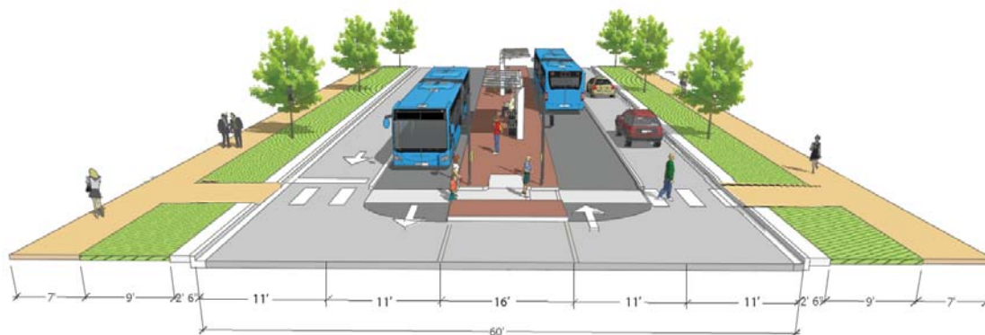
PROPOSED CROSS-SECTION AND DIMENSIONING OF COTTAGE GROVE AVENUE.
