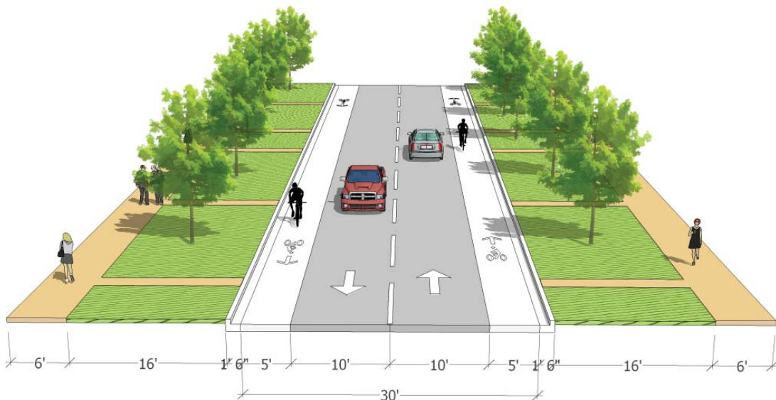
PROPOSED CROSS-SECTION AND DIMENSIONING OF ST LAWRENCE AVENUE
